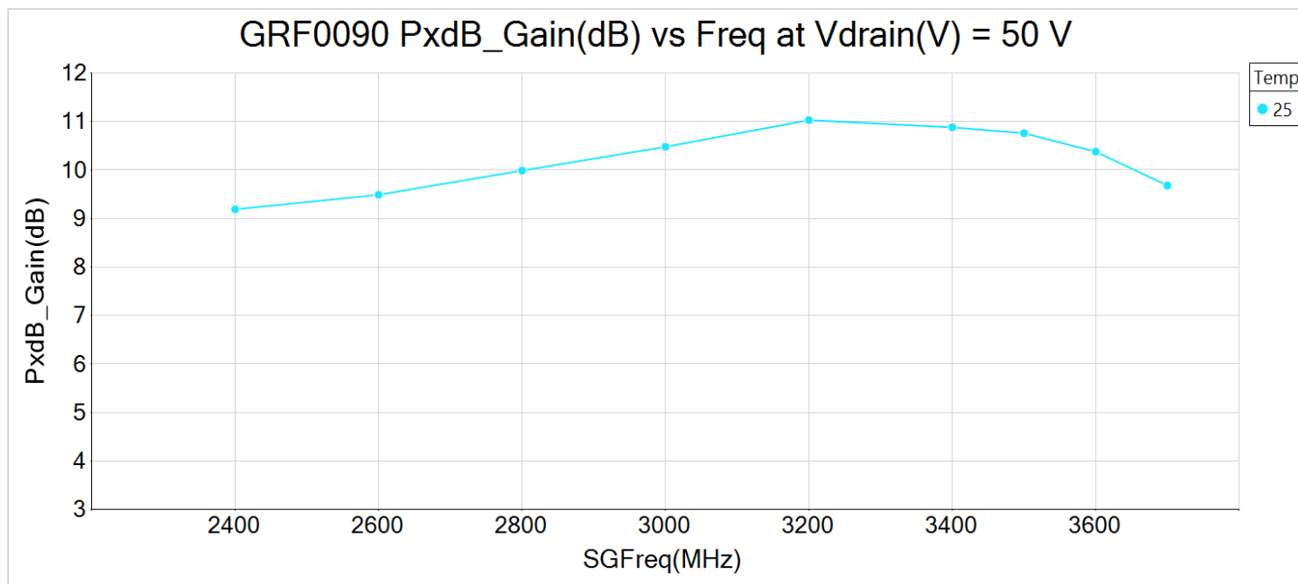
Gain vs. Frequency: 2.5 dB Compression
